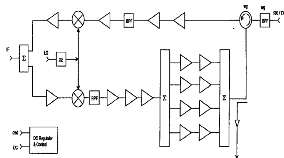
Figure 1. Crosslink T/R-Converter Block Diagram
