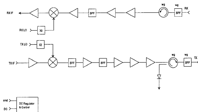
Figure 2. Gateway T/R-Converter Block Diagram
